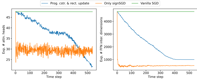
Fig. 2: The searching dynamics of different approaches. (Left) shows the expected number of attention heads. (Right) shows the FFN intermediate dimensions.
