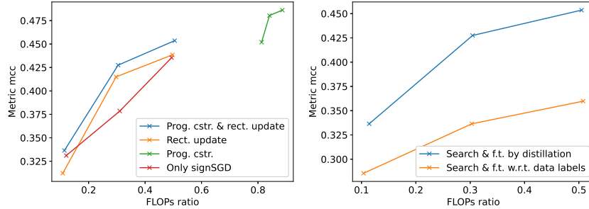
Fig. 3: (Left) shows the architecture accuracies under different approaches. (Right) shows the effect of knowledge distillation for searching and fine-tuning.
