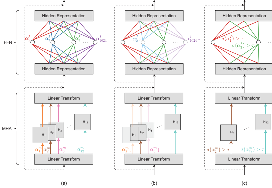
Fig. 1: An overview of the search method and search space of a BERT hidden layer, with multi-head attention block in the bottom and feed-forward block on the top. Dashed arrows represent skip connections. (a) The original network is initialized as the super-graph. An architecture parameter \alpha_i is assigned to each group of weights of the same color in the diagram. (b) Learning the \alpha_i w.r.t. the objective function. (c) Output the optimal sub-network by selecting \alpha that exceeds the threshold \tau .
